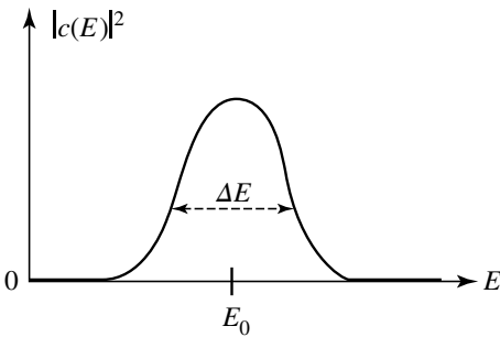
Figure 4: By superposing the stationary states |\varphi_E\rangle with the coefficients c(E) , we obtain a state |\psi\rangle of the system where the energy is not perfectly well-defined. The corresponding uncertainty \Delta E is given by the width of the curve that represents |c(E)|^2 . According to the fourth uncertainty relation, the evolution of the state |\psi(t)\rangle will be significant after a time \Delta t such that \Delta E \cdot \Delta t \gtrsim \hbar .
