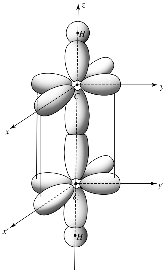
Figure 7: Schematic structure of the acetylene molecule C_2H_2 . For each carbon atom, two electrons are in the sp_z hybrid orbitals (cf. Fig. 6) and contribute to the C-H and C-C bonds ( \sigma bonds). In addition, two electrons are in the p_x and p_y orbitals and form additional bonds between the two carbon atoms ( \pi bonds, weaker than \sigma bonds), shown by the vertical lines in the figure. The C-C bond is therefore a “triple bond”.
