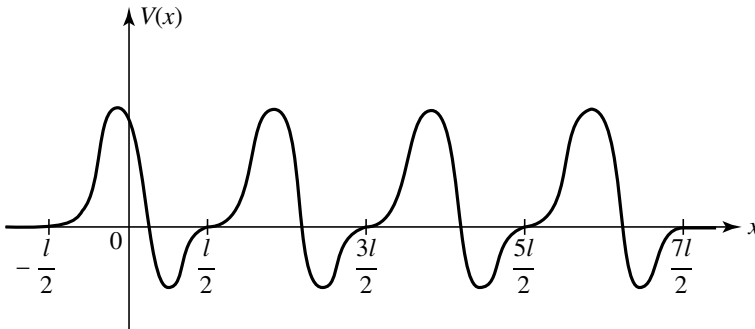
Figure 1: Potential V(x) having a periodic structure obtained by juxtaposing N times the same motif ( N = 4 in the figure).
