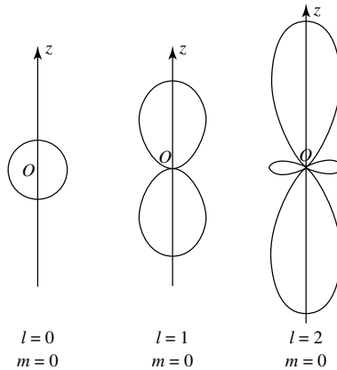
Figure 5: Angular dependence, Y_l^m(\theta, \varphi) , of some stationary wave functions of the hydrogen atom, corresponding to well-defined values of l and m . For each direction of polar angles \theta , \varphi , the value of |Y_l^m(\theta, \varphi)|^2 is recorded; a surface of revolution about the Oz axis is thus obtained. When l = 0 , this surface is a sphere centered at O ; it becomes more complicated for higher values of l .
