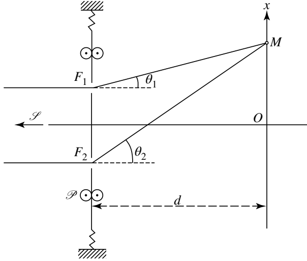
Figure 1: Diagram of a device using a movable plate \mathcal{P} whose momentum is measured before and after the passage of the photon to determine whether the photon passed through F_1 or through F_2 before arriving at point M on the screen.
