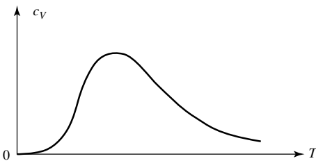
Figure 4: Specific heat c_V for a set of two-level systems. At high temperatures, c_V approaches zero because the energy spectrum has an upper bound.
