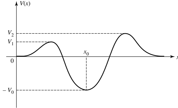
Figure 4: Potential well of depth -V_0 situated between two potential barriers of height V_1 and V_2 (assuming, for example, V_1 \leq V_2 ). Classically, there exist particle states whose energy is between -V_0 and V_1 that remain confined between the two barriers. In quantum mechanics, a particle whose energy is between 0 and V_1 can penetrate the barrier by the tunnel effect (§ 2-b- \beta of Complement H_1 ); consequently, the bound states always have energies between -V_0 and 0.
