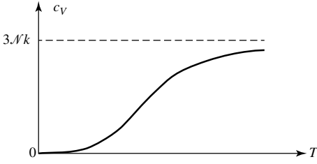
Figure 3: (Constant volume) specific heat c_V of a solid in Einstein's model. The high-temperature limit corresponds to the classical Dulong-Petit law.
