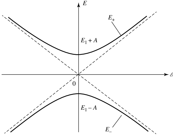
Figure 9: Influence of an electric field \mathcal{E} on the first two levels of the ammonia molecule (their spacing 2A in a zero field is due to the tunnel effect coupling). For weak \mathcal{E} , the molecule acquires a dipole moment proportional to \mathcal{E} , and the corresponding energy varies with \mathcal{E}^2 . For large \mathcal{E} , the dipole moment approaches a limit (corresponding to the nitrogen atom either above or below the plane of the hydrogen atoms), and the energy becomes a linear function of \mathcal{E} .
