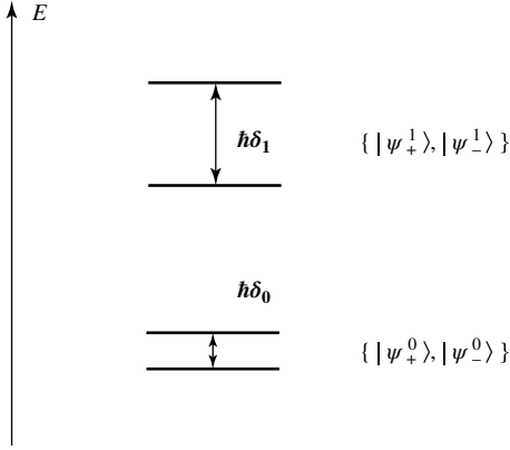
Figure 11: The tunnel effect removes the degeneracy of the energy levels shown in Figure 10. As one approaches the top of the barrier, this phenomenon becomes more important ( \delta_1 > \delta_0 ). |\psi_+^0\rangle , |\psi_-^0\rangle , |\psi_+^1\rangle , |\psi_-^1\rangle are the new stationary states.
