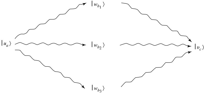
Figure 6: Different possible “paths” for the state vector of the system when the system is allowed to evolve freely (without undergoing any measurement) between the initial state |u_a\rangle and the final state |v_c\rangle . In this case, we must add together the probability amplitudes associated with these different paths, and not their probabilities.
