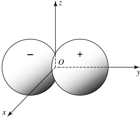
Figure 4: Angular dependence of a p_y orbital.
