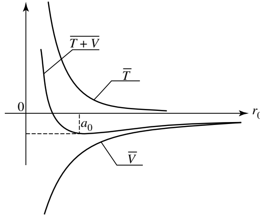
Figure 1: Variation with respect to r_0 (extension of the wave function) of the potential energy \bar{V} , the kinetic energy \bar{T} , and the total energy \bar{T} + \bar{V} of a hydrogen atom. The functions \bar{T} and \bar{V} vary inversely, so the total energy passes through a minimum value for some value of \bar{T} and \bar{V} . The corresponding value a_0 of r_0 gives the order of magnitude of the hydrogen atom's size.
