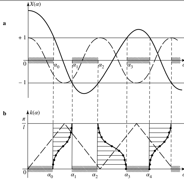
Figure 4: Variation with respect to \alpha of X(\alpha) = \text{Re}[F(\alpha)e^{i\alpha l}] (see Fig. 2) and of k(\alpha) = \frac{1}{l} \text{Arccos } X(\alpha) . The values of \alpha (that is, of the energy E ) associated with stationary states are obtained (if N \gg 1 ) by cutting the curve which represents k(\alpha) with the horizontal lines whose equations are y = p\pi/Nl ( p = 0, 1, 2, \dots, N - 1 ). The allowed bands are thus revealed (intervals \alpha_0 \leq \alpha \leq \alpha_1 , etc.); each includes N very close levels. The forbidden bands are represented by the shaded areas ( \alpha_1 < \alpha < \alpha_2 , etc...). The dashed-line curves correspond to the special case where V(x) = 0 (a free particle).
