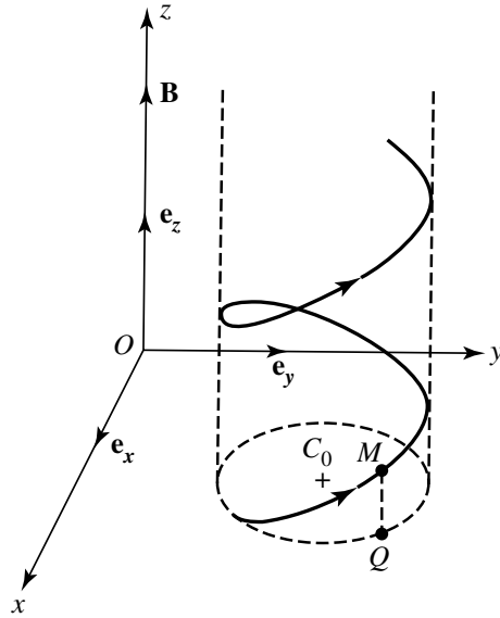
Figure 1: Classical trajectory of a charged particle in a uniform magnetic field parallel to Oz . The particle moves at constant velocity along a circular helix whose axis, parallel to Oz , passes through the point C_0 . The figure is drawn for q < 0 (the case of the electron), that is, \omega_c > 0 .
