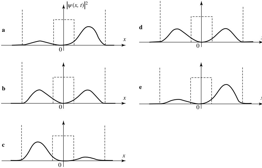
Figure 8: Evolution of a wave packet obtained by superposing the two stationary wave functions of Figure 7. The particle, initially, is in the right-hand well (fig. a ), tunnels into the left-hand well (fig. b ) and, after a certain time, becomes localized there (fig. c ); then it returns to the right-hand well (fig. d ) and the initial state (fig. e ), and so on.
