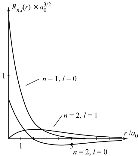
Figure 6: Radial dependence R_{n,l}(r) of wave functions associated with the first few levels of the hydrogen atom. When r \rightarrow 0 , R_{n,l}(r) behaves like r^l ; only the s states (for which l = 0 ) have a non-zero position probability at the origin.
