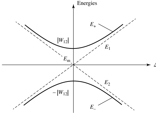
Figure 11: Variation of the energies E_+ and E_- as a function of the energy difference \Delta = (E_1 - E_2)/2 . In the absence of coupling, the levels cross at the origin (dashed straight lines). Under the effect of the non-diagonal coupling W , the two perturbed levels “repel each other” and we obtain an “anti-crossing”: the curves giving E_+ and E_- in terms of \Delta are branches of a hyperbola (solid lines in the figure) whose asymptotes are the unperturbed levels.
