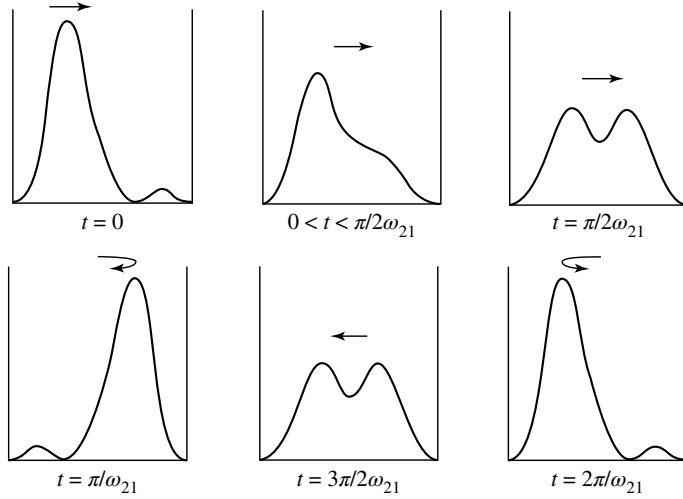
Figure 5: Periodic motion of a wave packet obtained by superposing the ground state and the first excited state of a particle in an infinite well. The frequency of the motion is the Bohr frequency \omega_{21}/2\pi .
