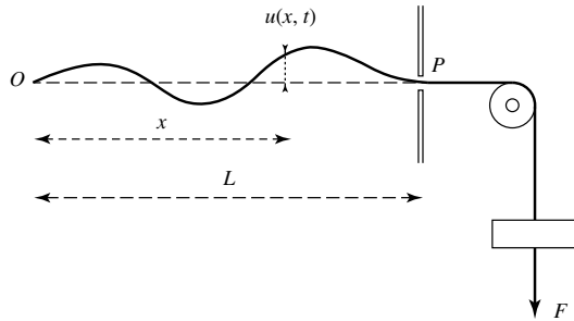
Figure 1: Vibrating string passing through two fixed points O and P and subjected to a tension F ; u(x, t) denotes the deviation with respect to the equilibrium position of the point of the string situated at a distance x from O .
