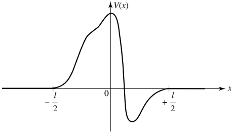
Figure 1: The potential V(x) under consideration varies in an arbitrary way within the interval -l/2 \leq x \leq l/2 and goes to zero outside this interval.
