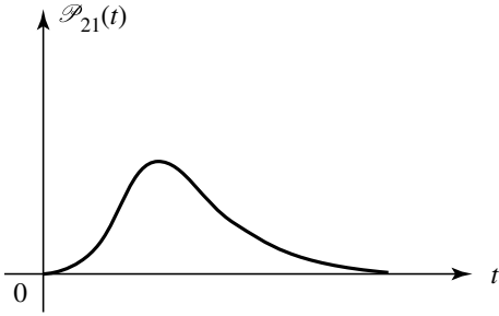
Figure 2: When the coupling is weak, oscillations between the states |\varphi_1\rangle and |\varphi_2\rangle do not have time to occur.
