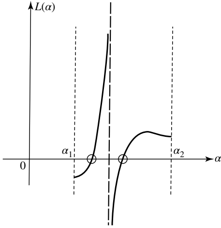
Figure 7: Variation of L(\alpha) with respect to \alpha in a forbidden band. The zeros of L(\alpha) give the stationary states which are localized on the edges of the lattice.
