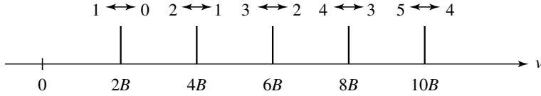
Figure 3: Frequencies appearing in the evolution of the mean value of the observable Z . Because of the selection rule \Delta l = \pm 1 , only the Bohr frequencies 2Bl (with l \geq 1 ), associated with two adjacent levels E_l and E_{l-1} in Figure 2, are observed.
