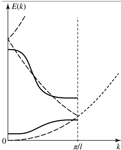
Figure 6: Variation of the energy with respect to the parameter k . The solid lines correspond to the energies for the first two allowed bands (the values of k which give the energy levels being equidistant inside the interval 0 \leq k \leq \pi/l ). The dashed lines correspond to the special case where the potential V(x) is zero (a free particle); the allowed bands are then contiguous, and there are no forbidden bands.
