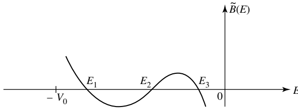
Figure 2: Graphical representation of the function \tilde{B}(E) . The zeros of \tilde{B}(E) give the values of E for which \varphi(x) is square-integrable (the situation in Figure 1c), that is, the energies E_1, E_2, E_3, \dots of the bound states; all these energies are included between -V_0 and 0.
