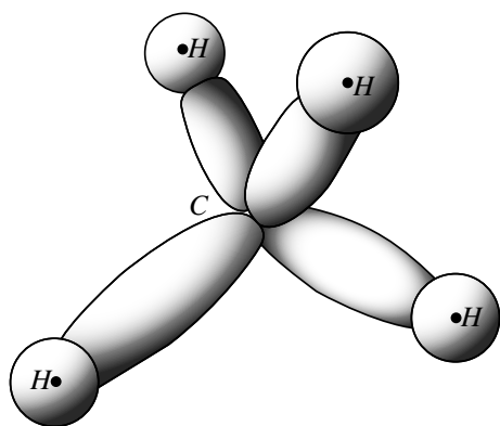
Figure 10: Schematic structure of the methane molecule. The sp^3 orbitals produce bonds arranged like the straight lines joining the center of a tetrahedron to its four corners (angles of 109^\circ 28' ).
