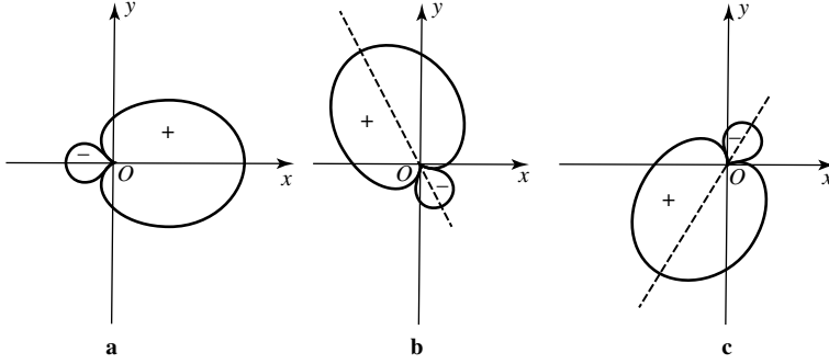
Figure 8: Angular dependence of the three orthogonal sp^2 orbitals. The \varphi_{n,s,p_x,p_y} , \varphi'_{n,s,p_x,p_y} and \varphi''_{n,s,p_x,p_y} orbitals can be transformed into each other by rotations through 120^\circ about Oz .
