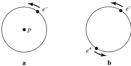
Figure 1: Schematic representation of the hydrogen (electron + proton system) and positronium (electron + positron system) atoms. Since the proton is much heavier than the electron, it is located practically at the center of mass of the hydrogen atom; the electron “revolves” about the proton at a distance a_0(\text{H}) . On the other hand, the positron is equal in mass to the electron; these particles therefore both revolve about their center of mass, the distance between them being a_0(\text{positronium}) = 2a_0(\text{H}) .
