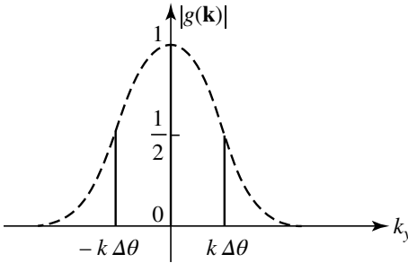
Figure 2: The three values chosen for k_y represent very schematically a peaked function |g(\mathbf{k})| (dashed line).
