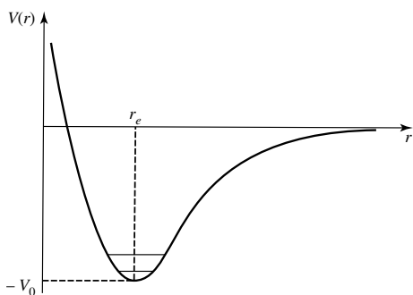
Figure 1: Variation of the interaction potential energy V(r) between the nuclei of a diatomic molecule as a function of the distance r between them. V(r) takes on its minimum value -V_0 at r = r_e . The first vibrational states are represented by the horizontal lines in the potential well.
