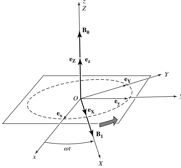
Figure 1: Oxyz is a fixed coordinate system. The static magnetic field \mathbf{B}_0 is directed along the Oz axis. The OXYZ system [the OX axis is in the direction of the field \mathbf{B}_1(t) ] rotates about Oz with the angular velocity \omega .
