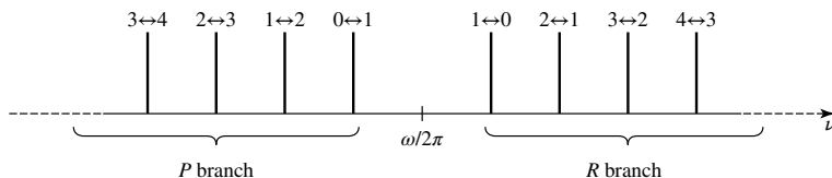
Figure 3: The vibrational-rotational spectrum for a heteropolar molecule. Since transitions between levels of Figure 2 with the same value of l are forbidden by the selection rules, no line has the pure vibrational frequency \frac{\omega}{2\pi} . Transitions in which the molecule passes from the level (v', l') to the level (v = v' - 1, l = l' - 1) correspond to frequencies \frac{\omega}{2\pi} + 2B(l + 1) (lines of the “R branch”). Transitions in which the molecule passes from the level (v', l') to the level (v = v' - 1, l = l' + 1) correspond to frequencies \frac{\omega}{2\pi} - 2B(l' + 1) (lines of the “P branch”). The different lines are labeled l' \leftrightarrow l in the figure.
