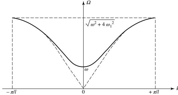
Figure 2: Dispersion relation giving the variation of the angular frequency of the vibrational normal modes with respect to the wave number k in the first Brillouin zone [-\pi/l, +\pi/l] . The dashed line corresponds to the case \omega = 0 .
