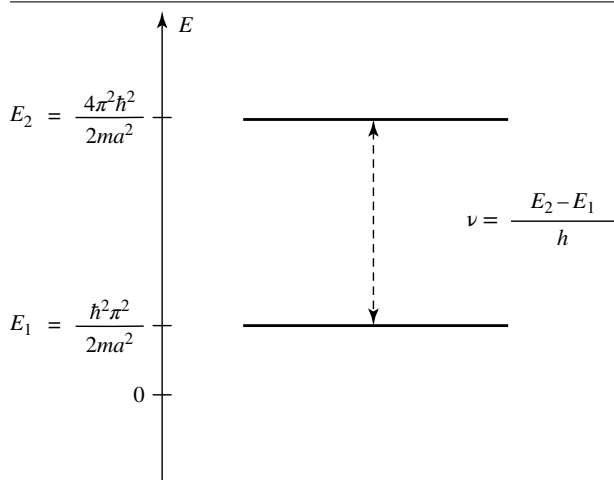
Figure 4: First energy levels obtained in the potential wells of Figure 3. The oscillation of the system in one of the two wells at the Bohr frequency \nu = (E_2 - E_1)/h represents the vibration of the molecule about one of its two classical equilibrium positions.
