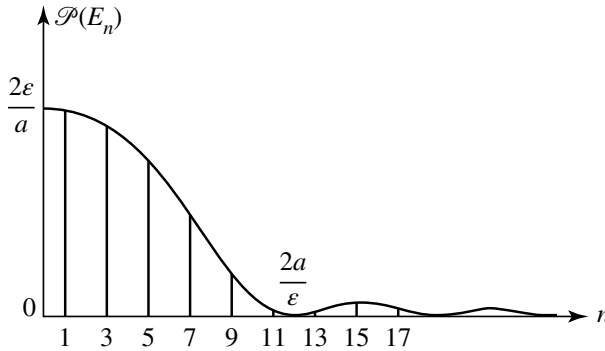
Figure 7: Variation with n of the probability \mathcal{P}(E_n) of finding the energy E_n after a measurement of the particle's position has yielded the result a/2 with an accuracy of \varepsilon ( \varepsilon \ll a ). The smaller \varepsilon , the greater the probability of finding high energy values.
