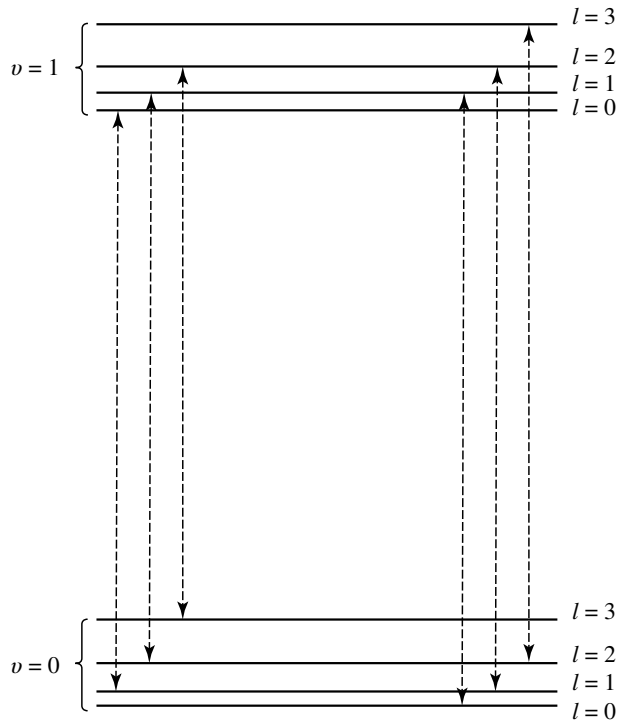
Figure 2: Diagram showing the first two vibrational levels ( v = 0 and v = 1 ) of a diatomic molecule and their rotational structure ( l = 0, 1, 2, \dots ). Within the limits of the approximations, this rotational structure is the same for the various vibrational levels. For a heteropolar molecule, the transitions represented by the vertical arrows in the figure yield the lines of the vibrational-rotational spectrum of the molecule. These lines fall in the infrared. These transitions obey the selection rule \Delta l = l' - l = \pm 1 .
