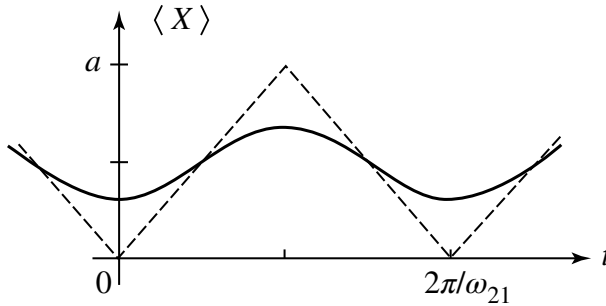
Figure 6: Time variation of the mean value \langle X \rangle corresponding to the wave packet's motion plotted in Figure 5. The dashed line represents the position of a classical particle moving with the same period. Quantum mechanics predicts that the center of the wave packet will turn back before reaching the wall, as explained by the action of the potential on the “edges” of the wave packet.
