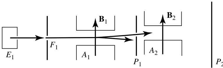
Figure 7: The first apparatus (a “source” composed of the furnace E_1 and the slit F_1 , plus a “polarizer” formed by the magnet A_1 and the pierced plate P_1 ) prepares the atoms in the state |+\rangle . The second one (an “analyzer” composed of the magnet A_2 and the plate P_2 ) measures the component \mathcal{S}_z . The result obtained is certain (+\hbar/2) .
