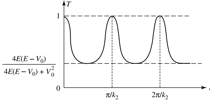
Figure 3: Variations of the transmission coefficient T of the barrier as a function of its width (the height V_0 of the barrier and the energy E of the particle are fixed). Resonances appear each time that l is an integral multiple of the half-wavelength \pi/k_2 , in region II.
