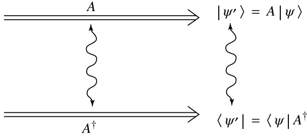
Figure 2: Definition of the adjoint operator A^\dagger of an operator A using the correspondence between kets and bras.
