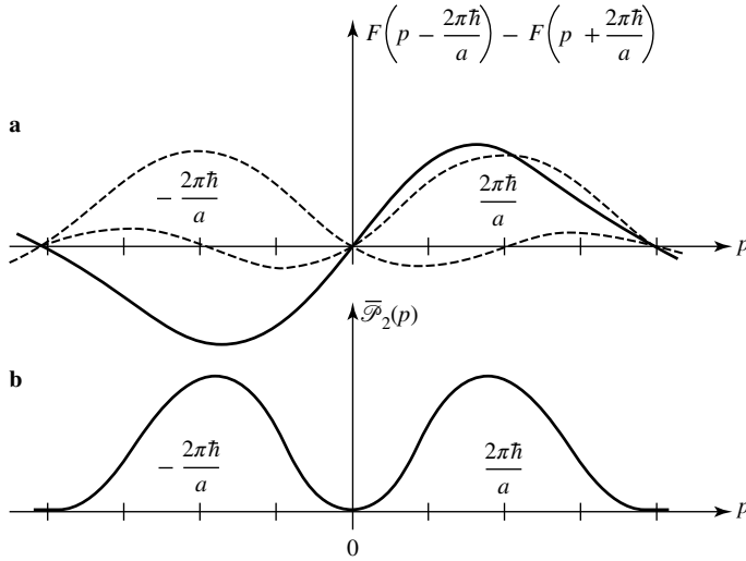
Figure 2: For the first excited level, the function \bar{\varphi}_2(p) is obtained by taking the difference between two functions F , which have the same width as in Figure 1-a but are now more widely separated (dash-line curves in figure a). The curve obtained in this way is the solid line in figure a. The probability density \bar{\mathcal{P}}_2(p) then has two maxima located in the neighborhood of p = \pm 2\pi\hbar/a (fig. b).
