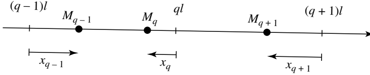
Figure 1: Infinite chain of oscillators; the displacement of the q th particle with respect to its equilibrium position ql is denoted by x_q .
