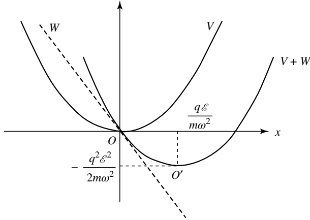
Figure 1: The presence of a uniform electric field has the effect of adding a linear term W to the potential energy V of the harmonic oscillator; the total potential V + W is then represented by a displaced parabola.
