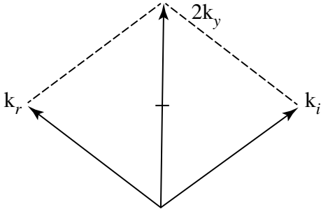
Figure 2: The sum of the probability currents associated with the incident and reflected waves yields a probability current parallel to Oy .
