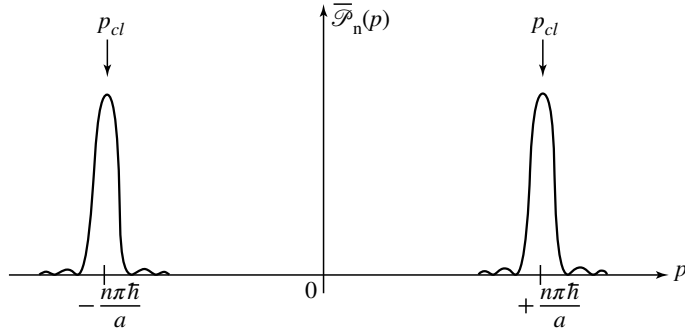
Figure 3: When n is large (a very excited level), the probability density has two pronounced peaks, centered at the values p = \pm n\pi\hbar/a , which are the momenta associated with the classical motion at the same energy.
