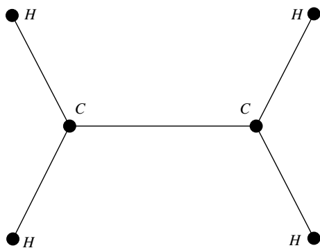
Figure 6: Plane structure of the ethylene molecule.
