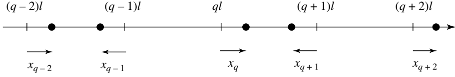
Figure 4: The modes k = \pm\pi/l are those in which two neighboring oscillators are completely out of phase; the coupling V strongly modifies their frequency.
