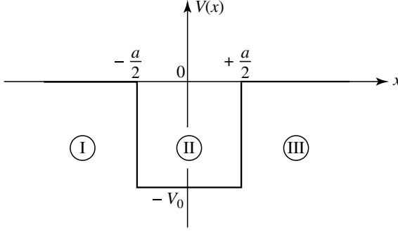
Figure 4: Square well potential.
