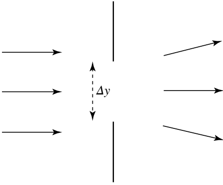
Figure 4: When the uncertainty \Delta y is decreased, the diffraction of the wave by the diaphragm increases the uncertainty \Delta k_y .
