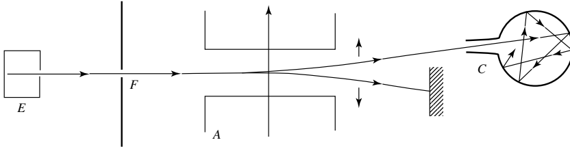
Figure 6: Schematic drawing of an experimental device which supplies cell C with atoms in the state |+\rangle .
