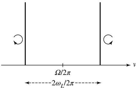
Figure 3: When the observation is carried out along the direction of the field \mathbf{B} , only two Zeeman components are obtained, circularly polarized in opposite directions and shifted by \pm\omega_L/2\pi .
