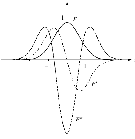
Figure 1: Shape of the Gaussian function F(z) and of its first and second derivatives F'(z) and F''(z) .
