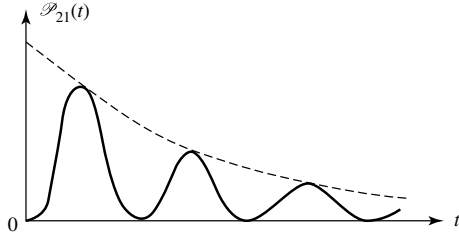
Figure 1: Effect of a strong coupling between a stable state |\varphi_2\rangle and an unstable state |\varphi_1\rangle . If the system is initially in the state |\varphi_2\rangle , the probability \mathcal{P}_{21}(t) of finding it in the state |\varphi_1\rangle at time t presents damped oscillations.
