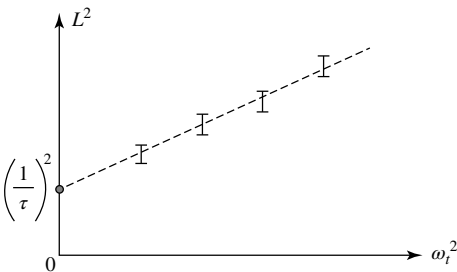
Figure 5: The extrapolation to \omega_1 = 0 of the squared half-width L of the resonance curve of Figure 4 gives the lifetime of the level being studied.
