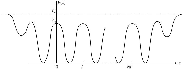
Figure 3: Variation with respect to x of the potential seen by an electron in a “one-dimensional crystal” and on its edges. Inside the crystal, the potential has a periodic structure; V(x) is maximum between the ions (barriers at x = 0, l, 2l, \dots ) and minimum at the positions of the ions (wells at x = l/2, 3l/2, \dots ). On the edges of the crystal, V(x) varies in a more or less complicated way over a distance comparable to l , then rapidly approaches a constant value V_e .
