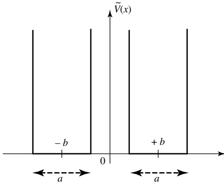
Figure 3: When the height V_0 of the potential barrier of Figure 2 is large, we have two practically infinite potential wells of width a whose centers are separated by a distance of 2b .
