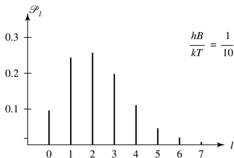
Figure 6: Population \mathcal{P}_l of the various rotational levels E_l at thermodynamic equilibrium. The fact that \mathcal{P}_l begins by increasing with l arises from the (2l + 1) -fold degeneracy of the levels E_l . When l becomes sufficiently large, the Boltzmann factor e^{-E_l/kT} prevails and is responsible for the decrease in \mathcal{P}_l .
