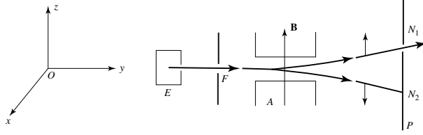
Figure 5: When we pierce a hole in the plate P at the position of the spot N_1 , the atoms that pass through this hole are all in the spin state |+\rangle . The Stern-Gerlach apparatus is then acting like a polarizer.
