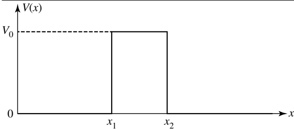
Figure 9: Potential barrier.
