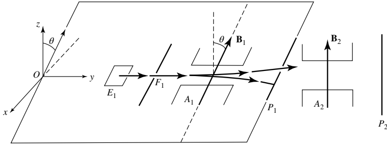
Figure 8: The first apparatus prepares the spins in the state |+\rangle_u ( \mathbf{u} is the unit vector of the xOz plane that makes an angle \theta with Oz ). The second one measures the \mathcal{S}_z component. The possible results are +\hbar/2 (probability \cos^2 \theta/2 ) and -\hbar/2 (probability \sin^2 \theta/2 ).
