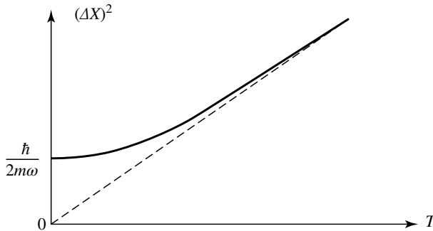
Figure 5: Variation with respect to the temperature T of (\Delta X)^2 , for a harmonic oscillator in thermodynamic equilibrium. When T \rightarrow \infty , \Delta X is identical to the classical value, shown by the dashed line; at low temperatures, quantum mechanical effects (Heisenberg uncertainty relation) prevent \Delta X from approaching zero.
