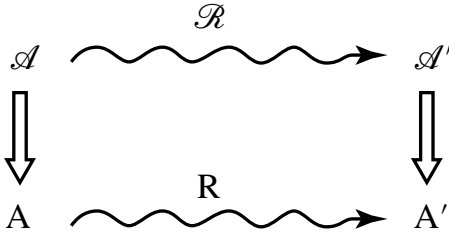
Figure 1: Behavior, under a rotation \mathcal{R} , of a classical physical quantity \mathcal{A} and of the associated observable A .
