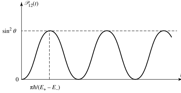
Figure 14: Variation with respect to time of the probability \mathcal{P}_{12}(t) of finding the system in the state |\varphi_2\rangle when it was initially in the state |\varphi_1\rangle . When the states |\varphi_1\rangle and |\varphi_2\rangle have the same unperturbed energy, the probability \mathcal{P}_{12}(t) can attain the value 1.
