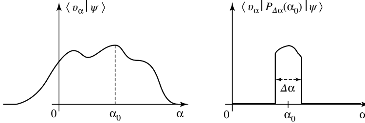
Figure 9: Illustration of the postulate of reduction of wave packets in the case of a continuous spectrum: one measures the observable A , with eigenvectors |v_\alpha\rangle and eigenvalues \alpha . The measurement device has a selectivity \Delta\alpha . If the value found is \alpha_0 to within \Delta\alpha , the effect of the measurement on the wave function \langle v_\alpha|\psi\rangle is to “truncate” it about the value \alpha_0 (to normalize the new wave function, it is obviously necessary to multiply it by a factor larger than 1).
