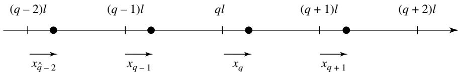
Figure 3: The lowest frequency mode ( k = 0 ; \Omega = \omega ) corresponds to a displacement of the system of oscillators “as a whole”. This is why its frequency does not depend on the coupling V .
