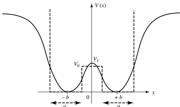
Figure 2: Variation with respect to x of the potential energy V(x) of the molecule. V(x) has two minima (classical equilibrium positions), separated by a potential barrier due to the repulsion for small |x| between the nitrogen atom and the three hydrogen atoms. The “square potential” used to approximate V(x) is shown in dashed lines.
