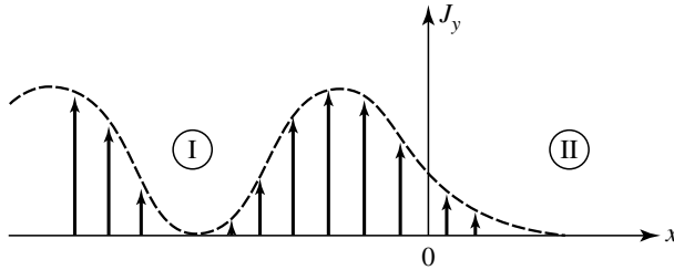
Figure 3: Because of the interference between the incident and reflected waves, the probability current in region I is an oscillatory function of x ; in region II, it decreases exponentially (evanescent wave).
