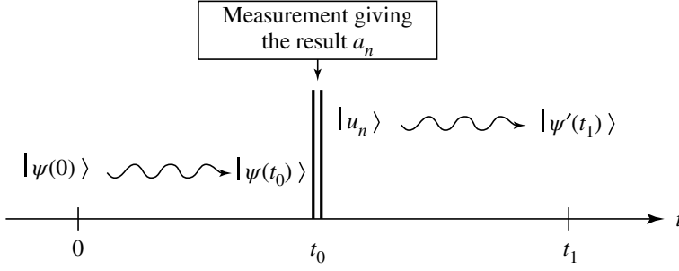
Figure 1: When a measurement at time t_0 of the observable A gives the result a_n , the state vector of the system undergoes an abrupt modification and becomes |u_n\rangle . This new initial state then evolves.
