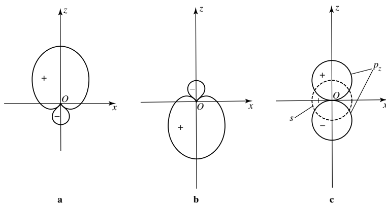
Figure 6: Angular dependence of the \varphi_{n,s,p_z}(\mathbf{r}) (fig. a) and \varphi'_{n,s,p_z}(\mathbf{r}) (fig. b), hybrid orbitals obtained from the \varphi_{ns}(\mathbf{r}) and \varphi_{np_z}(\mathbf{r}) orbitals, which have opposite parities (fig. c). A hybrid orbital can extend further in certain directions than the pure orbitals from which it is obtained.
