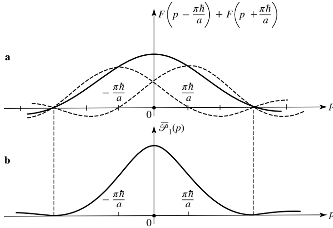
Figure 1: The wave function \overline{\varphi}_1(p) , associated in the \{|p\rangle\} representation with the ground state of a particle in an infinite well, is obtained by adding two diffraction functions F (dashed lines curves in figure a). Since the centers of these two functions F are separated by half their width, their sum has the shape represented by the solid-line curve in figure a. Squaring this sum, one obtains the probability density \overline{\mathcal{P}}_1(p) associated with a measurement of the momentum of the particle (fig. b).
