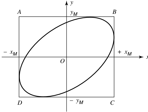
Figure 1: Projection of the classical trajectory of a particle in a two-dimensional harmonic potential onto the xOy plane; we obtain an ellipse inscribed in the rectangle ABCD .
