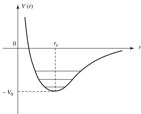
Figure 1: Form of the interaction potential between two atoms that can form a stable molecule. Classically, V_0 is the dissociation energy of the molecule and r_e , the distance between the two nuclei in the equilibrium position. In quantum mechanics, one obtains vibrational states (the horizontal lines inside the well) whose energies are all greater than -V_0 .
