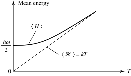
Figure 1: As a function of the temperature, variation of the mean energy of a quantum mechanical oscillator (solid line) compared with that of a classical oscillator (straight dashed line).
