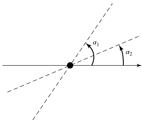
Figure 9: To write the classical equations of motion, we denote by \alpha_1 and \alpha_2 the angles formed by the planes of the two \text{CH}_2 groups with a fixed plane.
