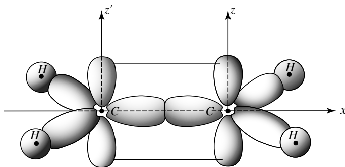
Figure 9: Schematic structure of the ethylene molecule C_2H_4 . The two carbon atoms form a double bond with each other: one \sigma bond due to sp^2 orbitals of the type of those shown in Figure 8 (the other two sp^2 hybrid orbitals at 120^\circ with this one form the C–H bonds), and one \pi bond, due to the overlapping of the p_z orbitals.
