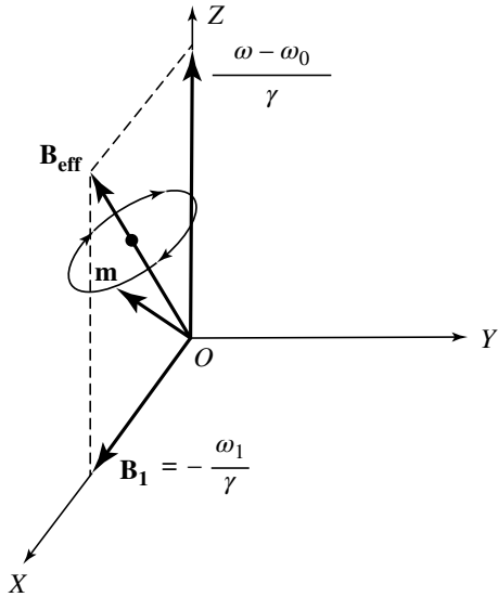
Figure 2: In the rotating reference frame OXYZ , the effective field \mathbf{B}_{\text{eff}} has a fixed direction, about which the magnetic moment \mathbf{m}(t) rotates with a constant angular velocity (precession in the rotating reference frame).
