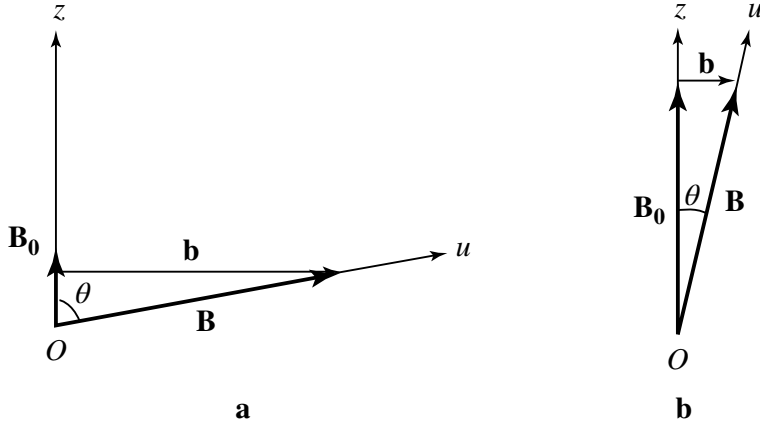
Figure 2: Relative disposition of the fictitious fields \mathbf{B}_0 , \mathbf{b} and \mathbf{B} in the case of strong coupling (fig. a) and weak coupling (fig. b).
