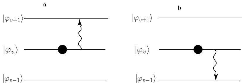
Figure 2: Absorption (fig. a) or emission (fig. b) of a photon by a heteropolar molecule going from the vibrational state |\varphi_v\rangle to the state |\varphi_{v+1}\rangle or |\varphi_{v-1}\rangle .
