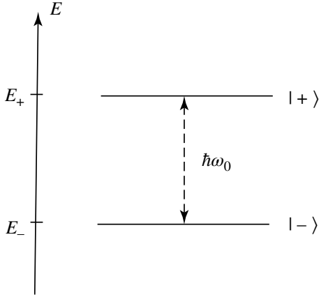
Figure 10: Energy levels of a spin 1/2, of gyromagnetic ratio \gamma , placed in a magnetic field B_0 parallel to Oz ; \omega_0 is defined by \omega_0 = -\gamma B_0 .
