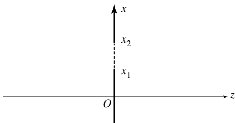
Figure 7: Schematic drawing of a device for measuring the abscissa x of a particle. Since the interval \{x_1, x_2\} is necessarily non-zero, such a device is always imperfectly selective.
