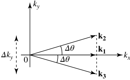
Figure 1: Arrangement of the wave vectors \mathbf{k}_1 , \mathbf{k}_2 and \mathbf{k}_3 associated with three plane waves that will be superposed to construct a two-dimensional wave packet.
