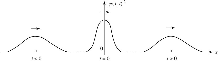
Figure 1: For negative t , the Gaussian wave packet decreases in width as it propagates. At time t = 0 , it is a “minimum” wave packet: the product \Delta x \cdot \Delta p is equal to \hbar/2 . Then, for t > 0 , the wave packet spreads again as it propagates.
