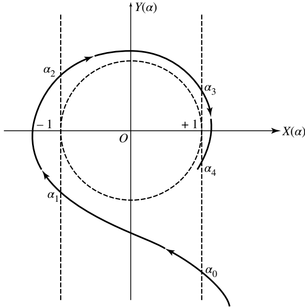
Figure 2: Variation with respect to \alpha of the complex number e^{i\alpha l}F(\alpha) = X(\alpha) + iY(\alpha) . Since |F(\alpha)| > 1 , the curve obtained in the complex plane falls outside the circle of unit radius centered at O . The following discussion shows that if |X(\alpha)| is less than 1, that is, if the value of \alpha chosen gives a point of the curve which is between the two vertical dashed lines of the figure, the corresponding energy falls in an “allowed band”; in the opposite case, it falls in a “forbidden band”.
