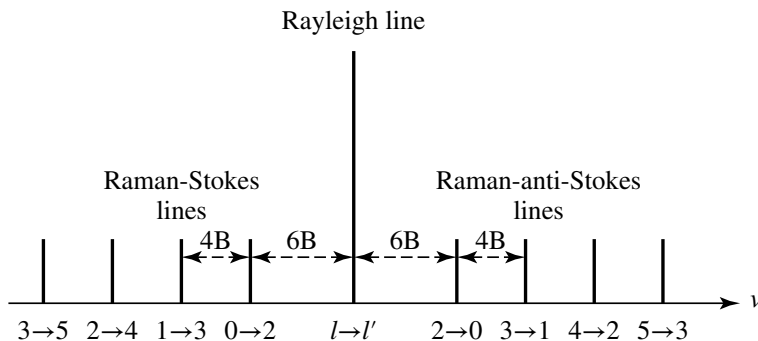
Figure 8: Raman rotational spectrum of a molecule. This molecule, initially in the rotational level E_l , inelastically scatters an incident photon of energy \hbar\Omega . After the scattering, the molecule has moved to the rotational level E_{l'} , and the energy of the photon is \hbar\Omega + E_l - E_{l'} (conservation of energy).
