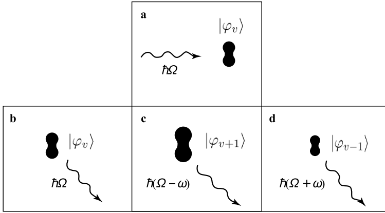
Figure 5: Schematic representation of the scattering of a photon of energy \hbar\Omega by a molecule which is initially in the vibrational state |\varphi_v\rangle (fig. a): Rayleigh scattering without a change in the vibrational state (fig. b); Stokes or anti-Stokes Raman scattering with a change in the molecule's state from |\varphi_v\rangle to |\varphi_{v+1}\rangle (fig. c) or to |\varphi_{v-1}\rangle (fig. d).
