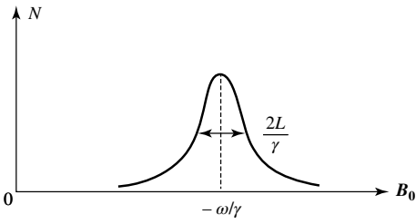
Figure 4: Resonance curve. To observe a resonance phenomenon, we perform an experiment in which n atoms are excited per unit time into the state |+\rangle . Under the effect of a field \mathbf{B}_1(t) , rotating at the frequency \omega/2\pi , the atoms undergo transitions towards the state |-\rangle . In the steady state, if we measure the number N of atoms which decay per unit time from the state |-\rangle , we obtain a resonant variation when we scan the static field B_0 about the value -\omega/\gamma .
