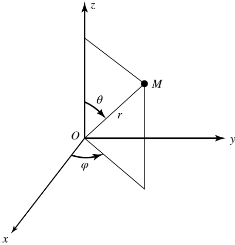
Figure 1: Definition of the spherical coordinates r, \theta, \varphi of an arbitrary point in space.
