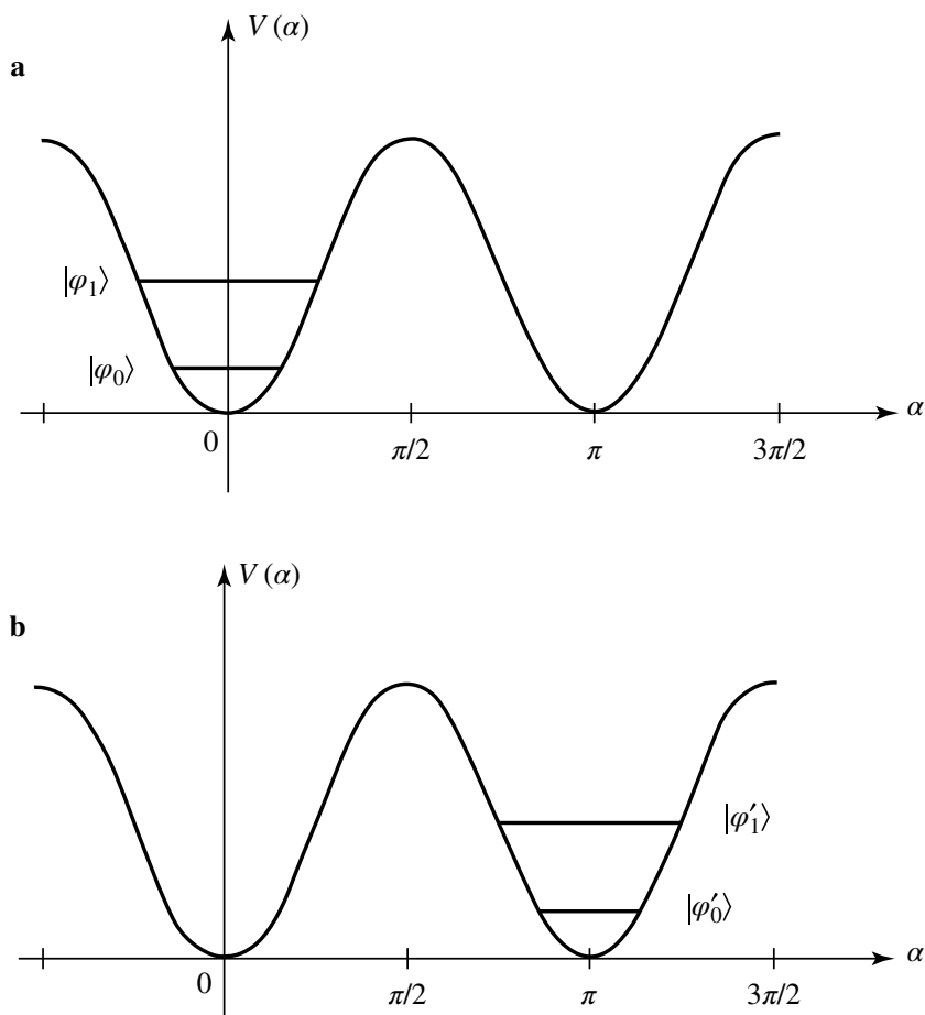
Figure 10: When one neglects the tunnel effect across the potential barriers at \alpha = \pi/2 and \alpha = 3\pi/2 , one can find torsional states of the molecule localized in the wells centered at \alpha = 0 (fig. a) and \alpha = \pi (fig. b).
