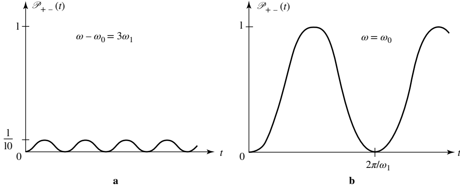
Figure 3: Variation with respect to time of the transition probability between the states |+\rangle and |-\rangle , under the effect of a rotating magnetic field B_1(t) . Outside resonance (fig. a), this probability remains small; at resonance (fig. b), however small the field B_1 , there exist times when the transition probability is equal to 1.
