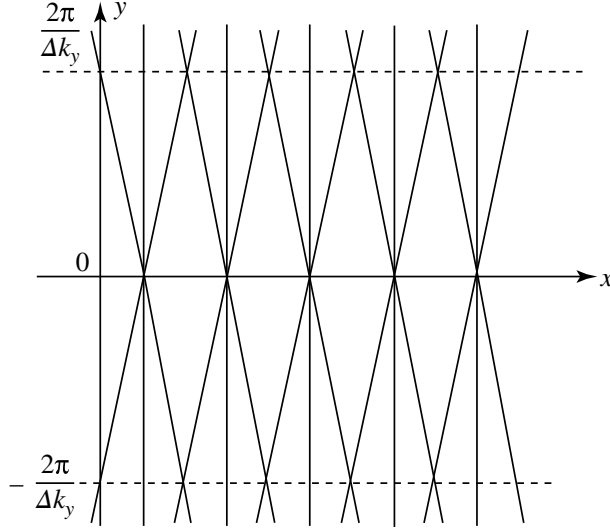
Figure 3: Equal phase planes of the three waves associated with the three \mathbf{k} vectors of Figure 1: these waves are in phase at y = 0 , but interfere destructively at y = \pm 2\pi/\Delta k_y .
