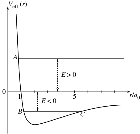
Figure 3: For a positive value of the energy E , the classical motion is not bounded. The spectrum of the quantum mechanical Hamiltonian H is therefore continuous for E > 0 , and the corresponding eigenfunctions are not normalizable. On the other hand, for negative E , the classical motion is limited to the interval BC . The spectrum of H is therefore discrete for E < 0 , and the corresponding eigenfunctions are normalizable.
