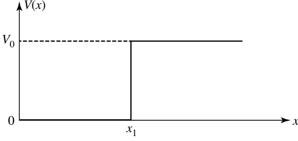
Figure 8: Potential step.
