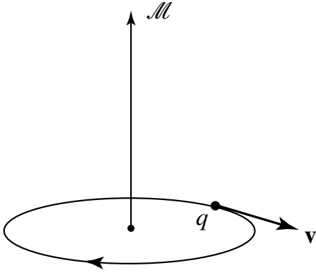
Figure 1: Classically, the motion of an electron in its orbit can be regarded as a current loop of magnetic moment \mathcal{M} .
