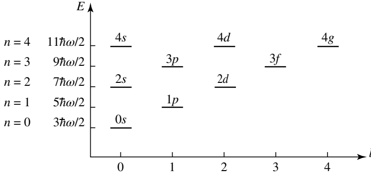
Figure 1: Lowest energy levels of the three-dimensional harmonic oscillator. When n is even, l can take on \frac{n}{2} + 1 values: l = n, n - 2, \dots, 0 . When n is odd, l can take on \frac{n+1}{2} values: l = n, n - 2, \dots, 1 . With the possible values of m ( -l \leq m \leq l ) taken into account, the degree of degeneracy of the level E_n is \frac{(n+1)(n+2)}{2} .
