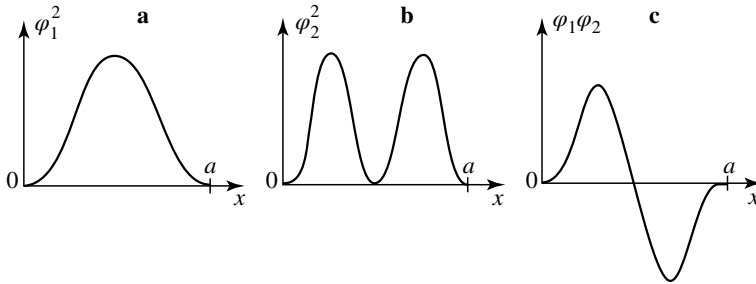
Figure 4: Graphical representation of the functions \varphi_1^2 (the probability density of the particle in the ground state), \varphi_2^2 (the probability density of the particle in the first excited state) and \varphi_1\varphi_2 (the cross term responsible for the evolution of the shape of the wave packet).
