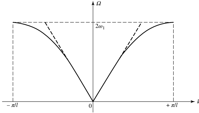
Figure 5: Dispersion relation for phonons (curve of Figure 2 for \omega = 0 ); the slope of the curve at the origin gives the speed of sound in the crystal.
