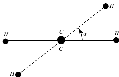
Figure 7: Torsion of the ethylene molecule (seen along the C – C axis): one of the CH 2 groups has rotated with respect to the other one through an angle \alpha about the C – C axis.
