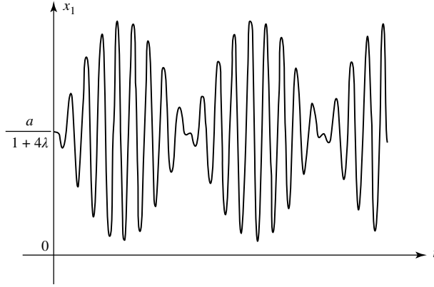
Figure 1: Oscillations of the position of particle (1), assumed to be motionless at its equilibrium position at t = 0 , particle (2) having an initial velocity. A beat phenomenon is produced between the two modes, and the amplitude of the oscillations of particle (1) varies over time.
