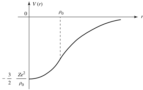
Figure 12: Form of the potential V(r) seen by a muon \mu^- attracted by a nucleus of radius \rho_0 situated at r = 0 . When r < \rho_0 , the variation of the potential is parabolic (if the charge density of the nucleus is uniform); when r > \rho_0 , V(r) varies like 1/r (Coulomb's law).
