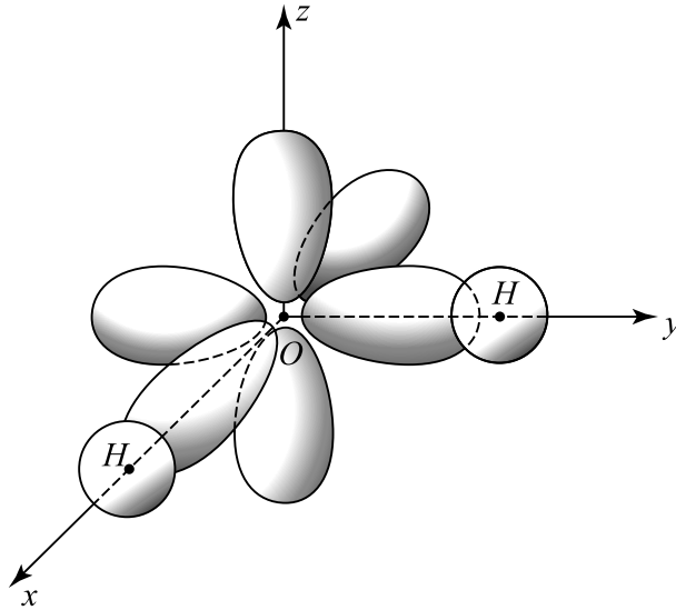
Figure 5: Schematic structure of the water molecule H_2O . The 2p_x and 2p_y orbitals yield bonds making an angle of approximately 90^\circ (the real angle is 104^\circ because of the electrostatic repulsion between the two protons).
