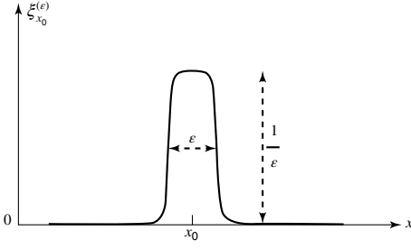
Figure 1: \xi_{x_0}^{(\varepsilon)}(x) is a function having a peak at x = x_0 (of width \varepsilon and amplitude 1/\varepsilon ), whose integral between -\infty and +\infty is equal to 1.
