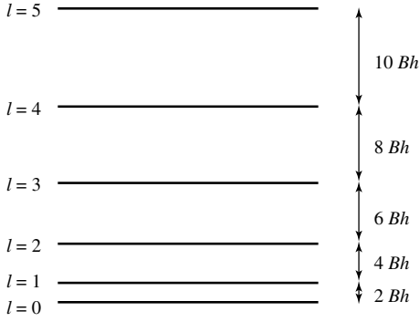
Figure 2: First levels of the rigid rotator, of energies:
