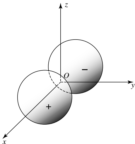
Figure 3: Angular dependence of a p_x orbital (the representation adopted is that of Figure 2-a).
