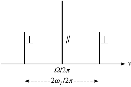
Figure 2: The Zeeman components of the resonance line of hydrogen observed in a direction perpendicular to the magnetic field \mathbf{B} (ignoring electron spin). We obtain a component of unshifted frequency \Omega/2\pi , polarized parallel to \mathbf{B} , and two components shifted by \pm\omega_L/2\pi , polarized perpendicularly to \mathbf{B} .
