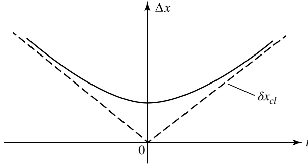
Figure 2: Variation in time of the width \Delta x of the wave packet of Figure 1. For large t , \Delta x approaches the dispersion \delta x_{cl} of the positions of a group of classical particles which left x = 0 at time t = 0 with a velocity dispersion \Delta p/m .
