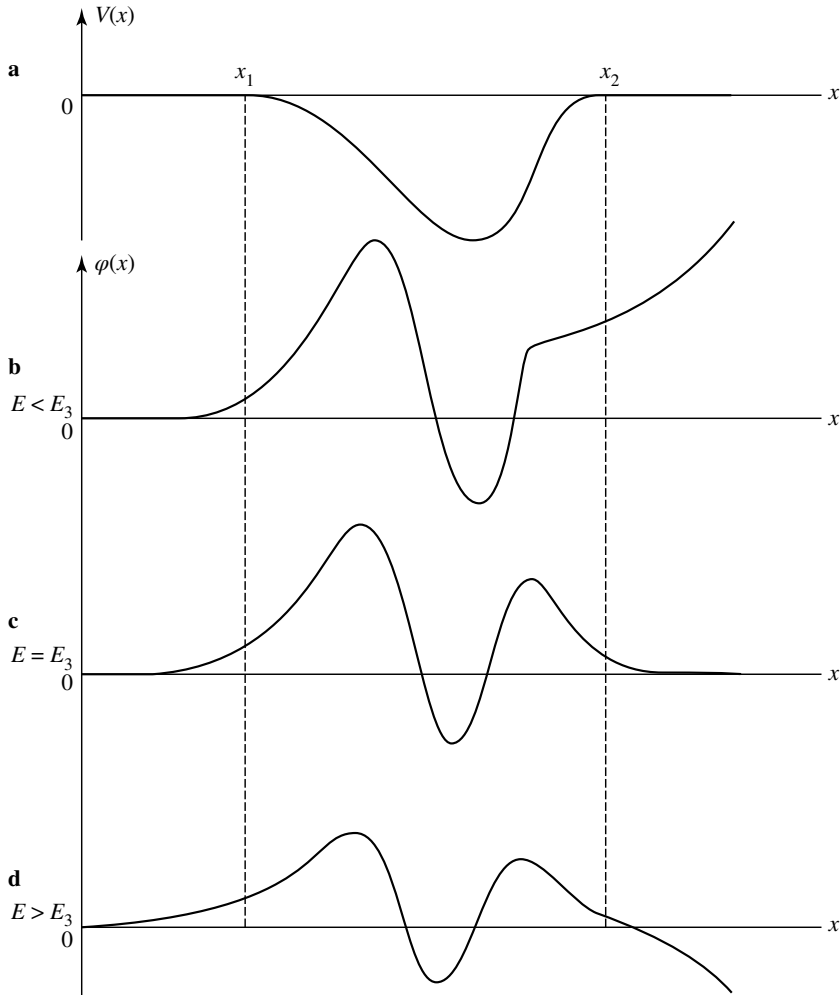
Figure 1: Potential well (fig. a) situated between the points x = x_1 and x = x_2 . We choose a solution \varphi(x) of the eigenvalue equation of H which, for x < x_1 , approaches zero exponentially when x \rightarrow -\infty . We then extend this solution to the entire x -axis. For an arbitrary energy value E , \varphi(x) diverges like \tilde{B}(E)e^{\rho x} when x \rightarrow +\infty : figure b represents the case where \tilde{B}(E) > 0 ; figure d, that where \tilde{B}(E) < 0 . However, if the energy E is chosen so as to make \tilde{B}(E) = 0 , \varphi(x) approaches zero exponentially when x \rightarrow +\infty (fig. c), and \varphi(x) is square-integrable.
