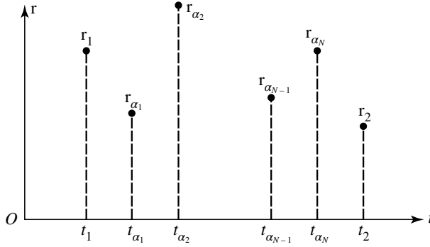
Figure 3: Diagram associated with a “spacetime path”: one picks N intermediate times t_{\alpha_i} ( i = 1, 2, \dots, N ) evenly spaced between t_1 and t_2 , and chooses for each of them a value of \mathbf{r} .
