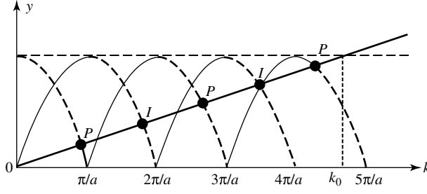
Figure 5: Graphic solution of equation (42), giving the energies of the bound states of a particle in a square well potential. In the case shown in the figure, there exist five bound states, three even (associated with the points P of the figure), and two odd (points I).
