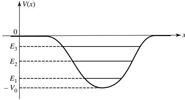
Figure 3: Schematic representation of the bound states of a particle in a potential well. For each of these stationary states, one draws a horizontal line whose ordinate is equal to the energy of the corresponding level. The ends of this line are the points of intersection with the curve representing the potential V(x) . The line is confined to the region of classical motion for the same energy, and gives an idea of the extension of the wave function.
