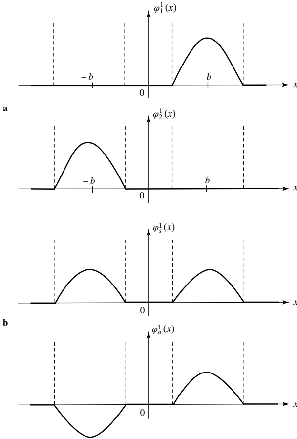
Figure 5: The states \varphi_1^1(x) and \varphi_2^1(x) , shown in figure a , are stationary states with the same energy, respectively localized in the right-hand well and the left-hand well of Figure 3. To use the symmetry of the problem, it is more convenient to choose as stationary states the symmetrical state \varphi_s^1(x) and the antisymmetrical state \varphi_a^1(x) , linear combinations of \varphi_1^1(x) and \varphi_2^1(x) (figure b )
