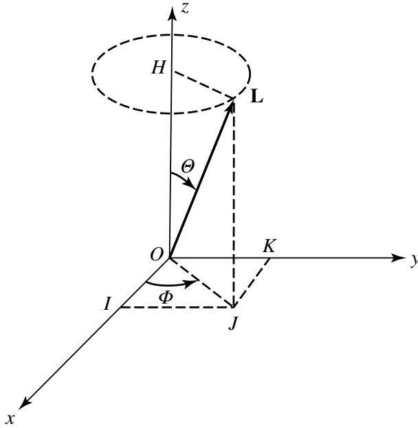
Figure 3: A classical model for the orbital angular momentum of a particle in a state |l, m\rangle . We assume that the distance |OL| and the angle \Theta are known, but that \Phi is a random variable whose probability density is constant inside the interval [0, 2\pi] . The classical mean values of the components of OL , as well as those of the squares of these components, are then equal to the corresponding quantum mechanical mean values.
