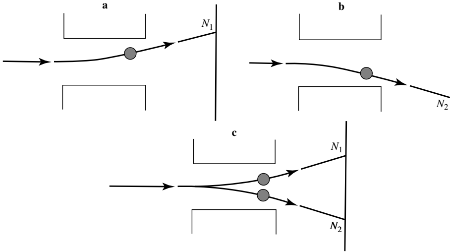
Figure 9: When the spin is in the state |+\rangle (fig. a) or |-\rangle (fig. b), the center of the wave packet follows a well-defined trajectory which can be calculated classically. When the spin state is a linear superposition of |+\rangle and |-\rangle , the wave packet splits into two parts and it is no longer possible to say that the atom follows a classical trajectory (despite the fact that the spread of each of the packets is much smaller than the characteristic dimensions of the problem).
