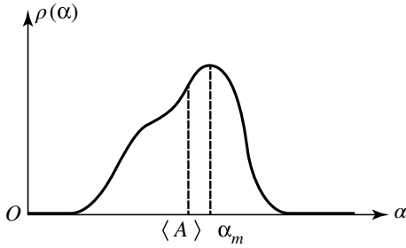
Figure 2: Variation with respect to \alpha of the probability density \rho(\alpha) . The mean value \langle A \rangle is the abscissa of the center of gravity of the area under the curve (it does not necessarily coincide with the abscissa \alpha_m of the maximum of the function).
