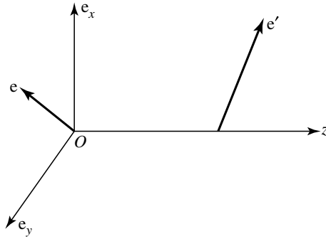
Figure 5: A simple experiment which illustrates the difference between a linear superposition and a statistical mixture of states. If all the incident photons are in the polarization state:
