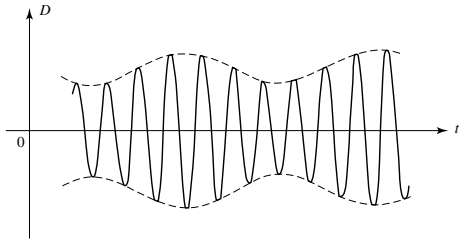
Figure 3: The vibration of a molecule modulates the amplitude of the oscillating electric dipole induced by an incident light wave.
