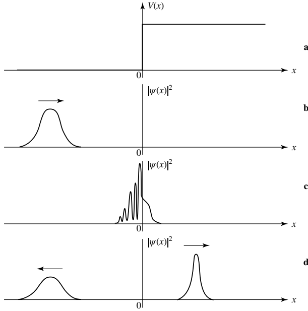
Figure 1: Behavior of a wave packet at a potential step, in the case E > V_0 . The potential is shown in figure a . In figure b , the wave packet is moving towards the step. Figure c shows the wave packet during the transitory period in which it splits in two. Interference between the incident and reflected waves are responsible for the oscillations of the wave packet in the x < 0 region. After a certain time (fig. d ), we find two wave packets. The first one (the reflected wave packet) is returning towards the left; its amplitude is smaller than that of the incident wave packet, and its width is the same. The second one (the transmitted wave packet) propagates towards the right; its amplitude is slightly greater than that of the incident wave packet, but it is narrower.
