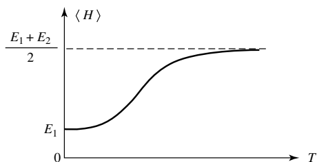
Figure 2: Mean energy of a quantum mechanical system with two energy levels E_1 and E_2 , in thermodynamic equilibrium at a temperature T .
