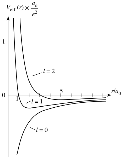
Figure 2: Shape of the effective potential V_{\text{eff}}(r) for the first values of l in the case where V(r) = -e^2/r . When l = 0 , V_{\text{eff}}(r) is simply equal to V(r) . When l takes on the values 1, 2, etc., V_{\text{eff}}(r) is obtained by adding to V(r) the centrifugal potential l(l+1)\hbar^2/2\mu r^2 , which approaches +\infty when r approaches zero.
