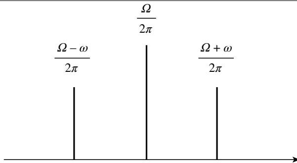
Figure 4: Spectrum of the oscillations shown in Figure 3. In addition to the central line, whose frequency is the same as that of the incident light wave (Rayleigh line), two shifted lines appear (the Stokes and anti-Stokes Raman lines). The frequency shift is equal to the vibrational frequency of the molecule.
