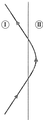
Figure 4: The penetration of the particle into region II leads to a lateral shift upon reflection.
