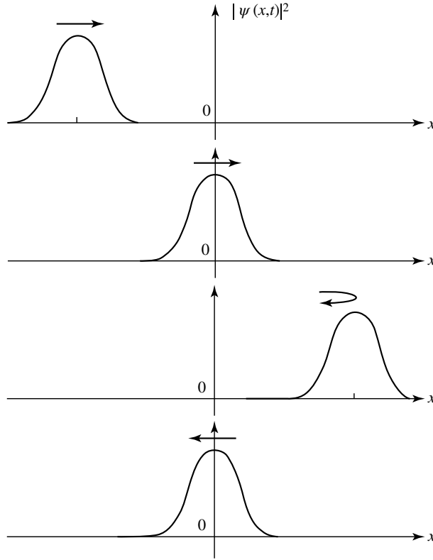
Figure 2: Motion of the Gaussian wave packet associated with an |\alpha\rangle state: under the effect of the parabolic potential V(x) , the wave packet oscillates without becoming distorted.
