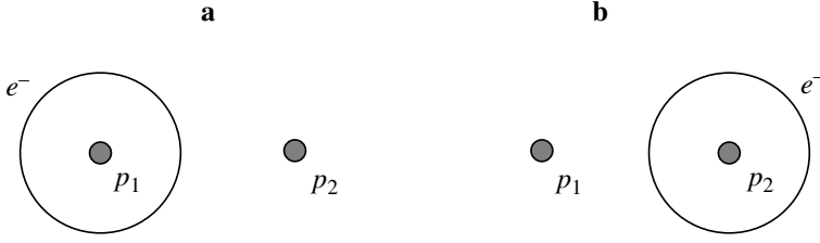
Figure 13: In the H_2^+ ion, the electron could logically be localized either around the proton p_1 (fig. a) or around the proton p_2 (fig. b). In the ground state of the ion, the wave function of the electron is a linear superposition of the wave functions associated with figures a and b. Its probability of presence is symmetrical with respect to the plane bisecting p_1p_2 .
