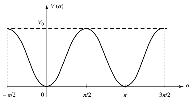
Figure 8: The potential energy of the molecule depends on the torsion angle \alpha ; V(\alpha) is minimal for \alpha = 0 and \alpha = \pi (planar structures).
