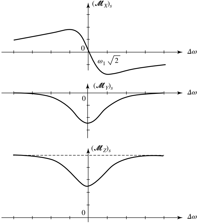
Figure 7: Variation with respect to \Delta\omega = \omega - \omega_0 of the stationary values of the components of \mathcal{M} in the rotating frame. One obtains a dispersion curve for (\mathcal{M}_X)_s and absorption curves for (\mathcal{M}_Y)_s and (\mathcal{M}_Z)_s . The three curves have the same width, 2\sqrt{\omega_1^2 + (1/T_R)^2} , which increases with \omega_1 . They have been drawn assuming that \omega_1 = 1/T_R ("half-saturation").
