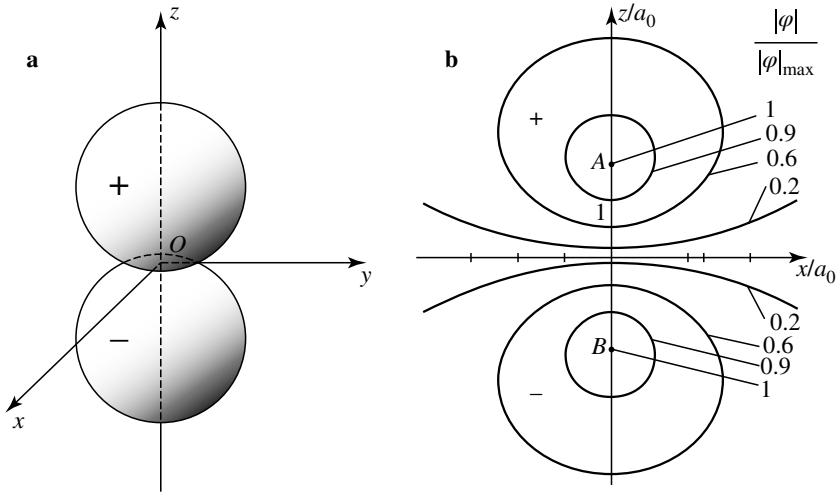
Figure 2: Two possible representations of a p_z orbital ( l = 1, m = 0 ) fig. a: angular dependence of this orbital. With r fixed, we display |\varphi_{n,l=1,m=0}(r, \theta, \varphi)| for each direction \theta, \varphi . Thus we obtain two spheres, tangential at O to the xOy plane. The sign indicated on each of them is that of the wave function (which is real). fig. b: cross sections in the xOz plane of a family of surfaces, each one corresponding to a given value for |\varphi_{n,l=1,m=0}(r, \theta, \varphi)| [we have chosen values equal to 0.2, 0.6, 0.9 times the maximum value of |\varphi| at points A and B ]. These are surfaces of revolution about Oz . The sign indicated is that of the wave function (which is real). Unlike the one in figure a, the representation in figure b depends on the radial part of the wave function (the one chosen here corresponds to the n = 2 state of the hydrogen atom).
