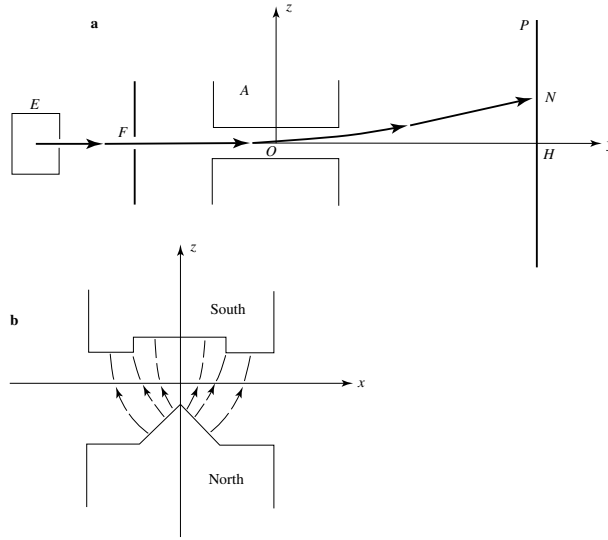
Figure 1: Schematic diagram of the Stern-Gerlach experiment. Figure a shows the trajectory of a silver atom emitted from the high-temperature furnace E . This atom is deflected by the gradient of the magnetic field created by the electromagnet A and then condenses at N on plate P .
